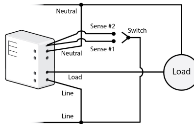
Dual Momentary
