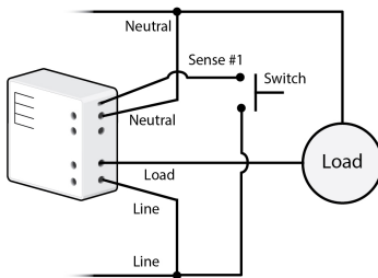
Single Momentary
